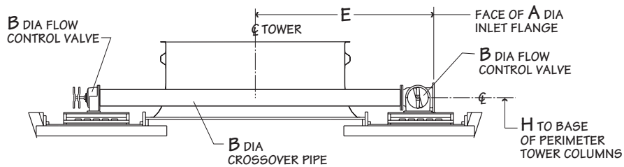
Section-Distribution System
