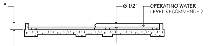
Section-Flat Slab Basin
