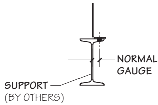
SECTION A
