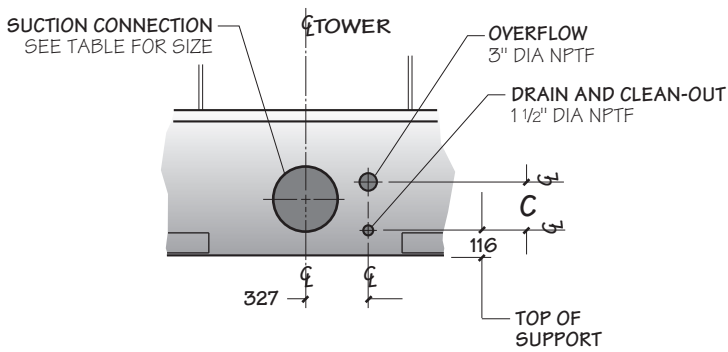
DRAIN AND OVERFLOW CONNECTION OPTION
