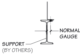
SECTION A
