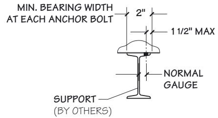
VIEW B
