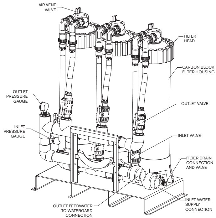
Triple Housing (WG037, WG061, WG073 and WG091)
