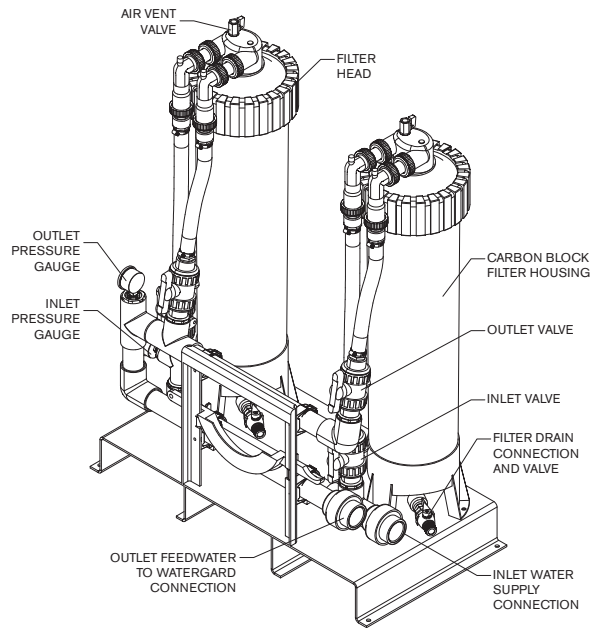
Double Housing (WG049 and WG055)
