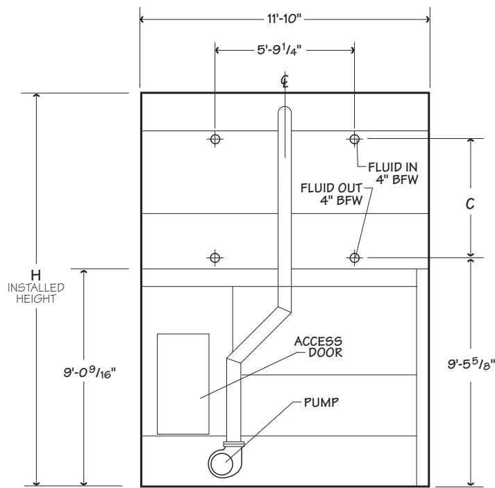
SIDE ELEVATION
