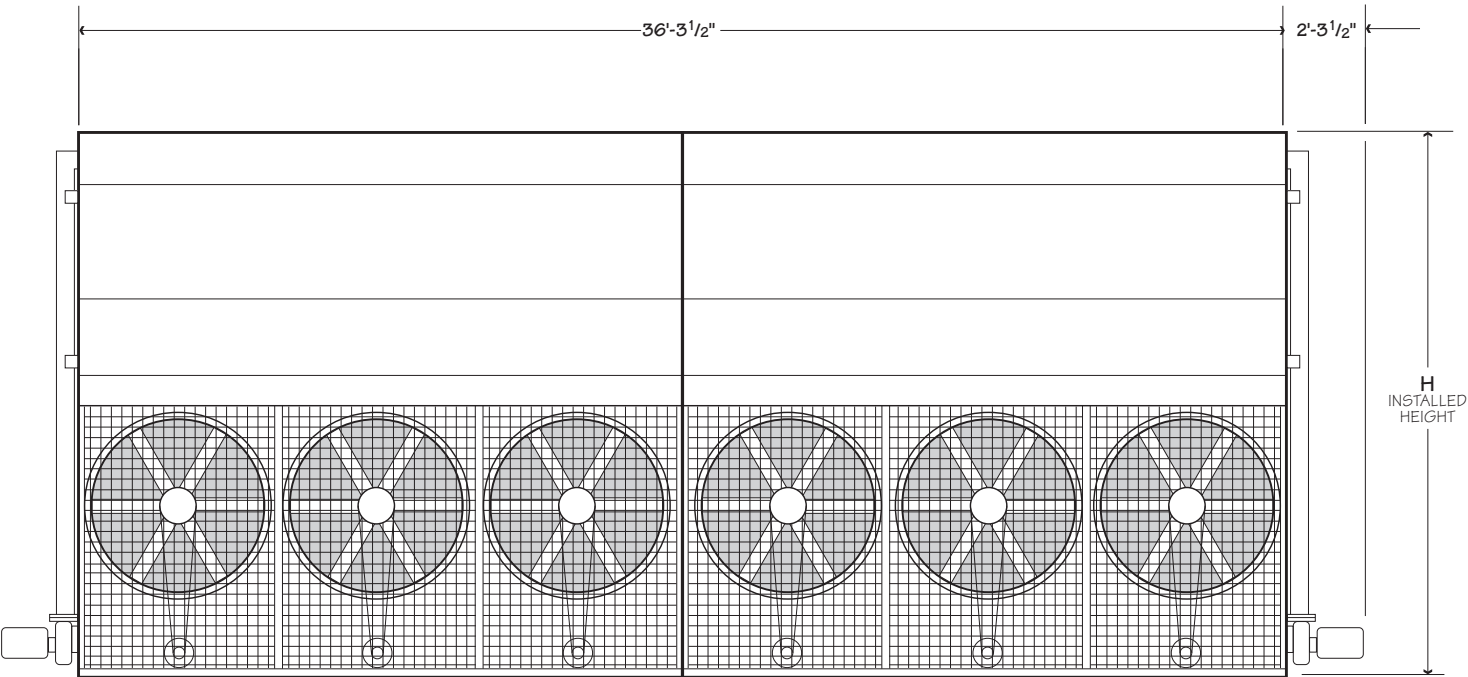
AIR INLET ELEVATION
