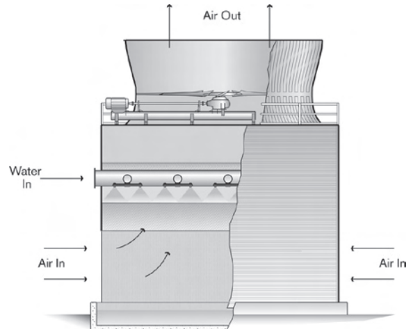
Figure 8 — Induced draft counterflow tower.
