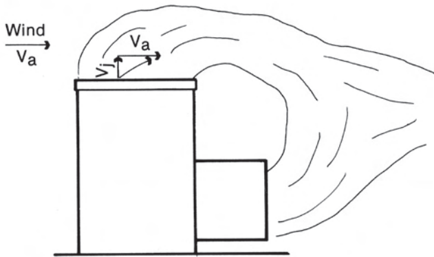
Figure 36 — Recirculation potential in a forced draft cooling tower.
