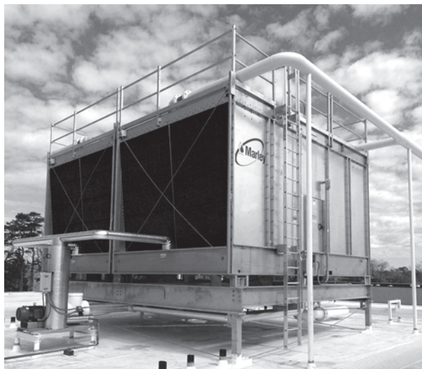
Figure 51 — Factory-assembled towers of stainless steel construction are utilized in corrosive areas.
