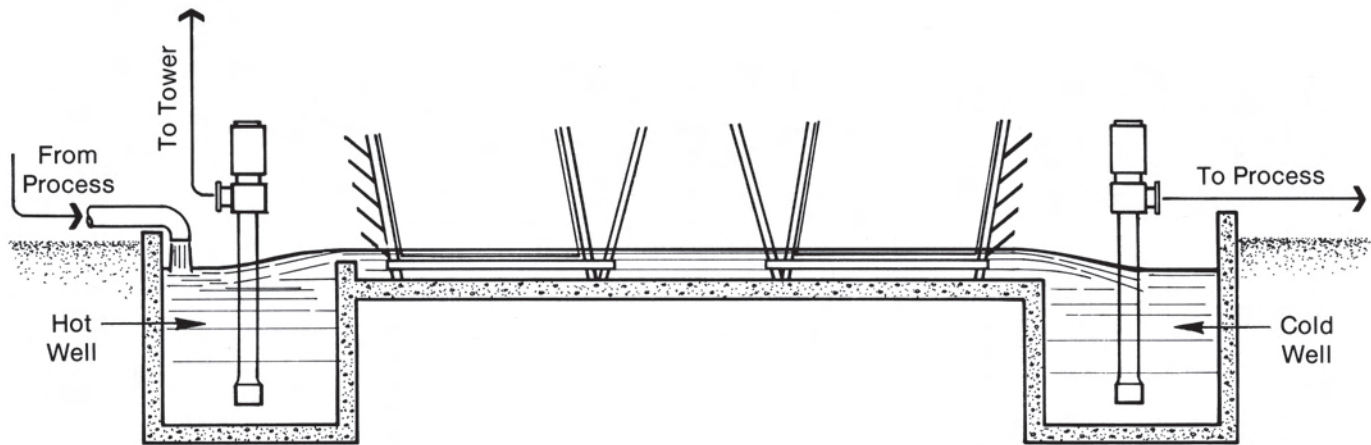
Figure 116 — Wier by-pass arrangement to control hot water temperature to tower.
