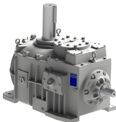
M Series Geareducer
