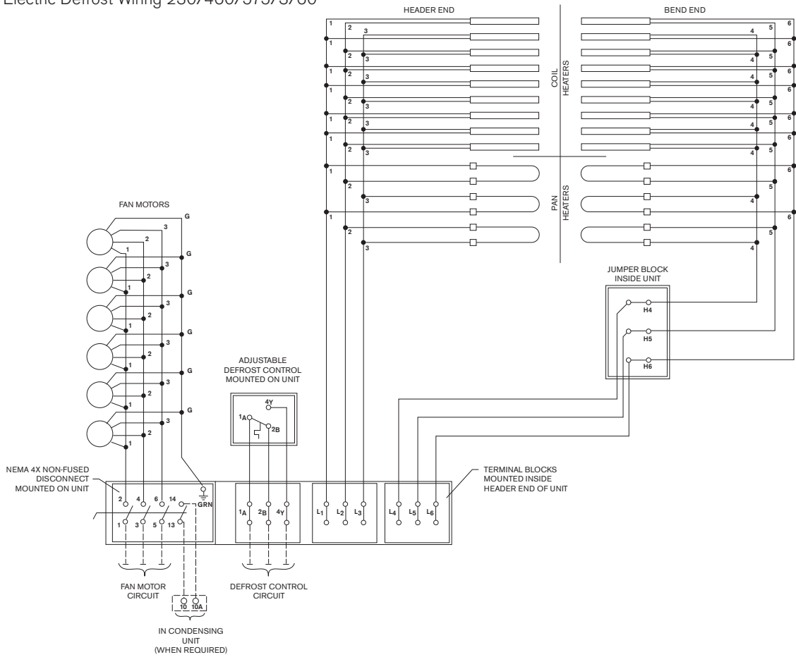
FIGURE 8 Electric Defrost Wiring 230/3/60
