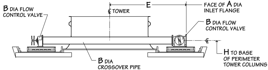
SECTION-DISTRIBUTION SYSTEM
