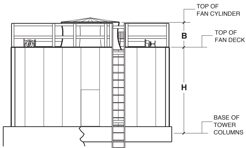
ENDWALL ELEVATION
