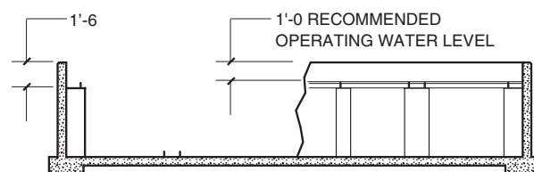
DEEP BASIN SECTION
