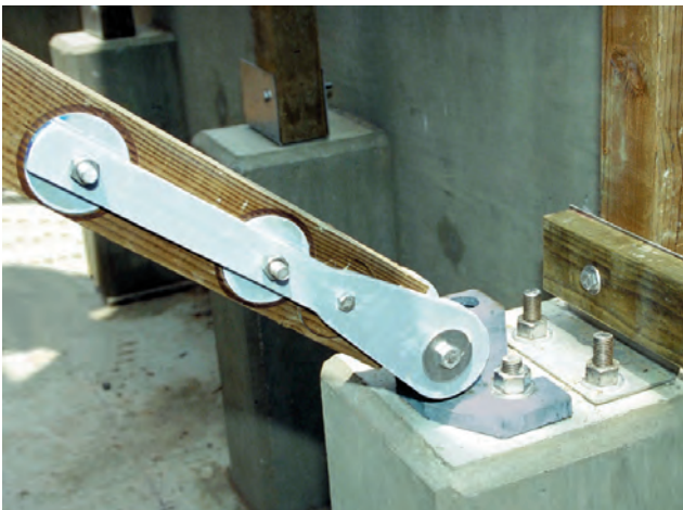
Diagonal and Column Anchorage
