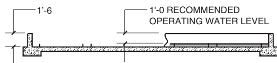
FLAT BASIN SECTION
