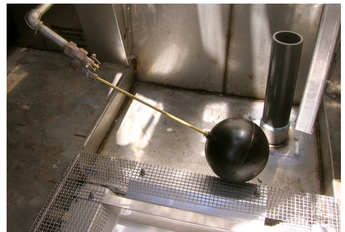
Inside the collection basin showing the makeup valve and overflow.
