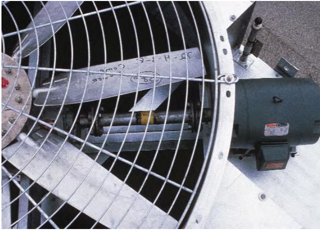
The fan and fan motor on a counterflow cooling tower
