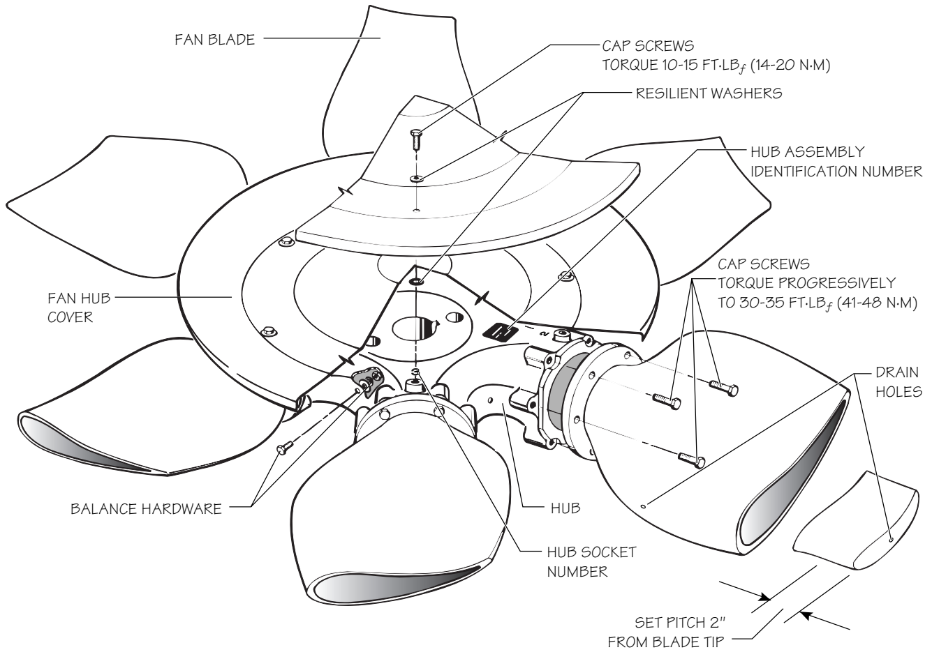
Figure 1 –Typical Fan Assembly
