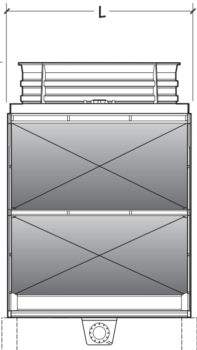
AIR INLET ELEVATION
