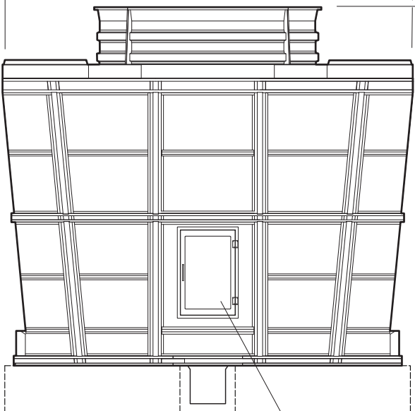
SIDE ELEVATION
