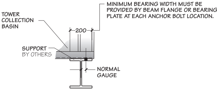
VIEW A
