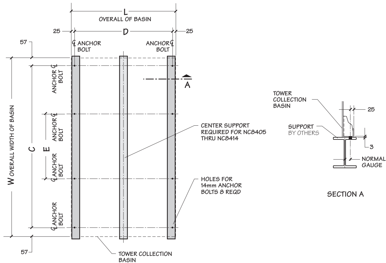
SUPPORTING STEEL SINGLE CELL
