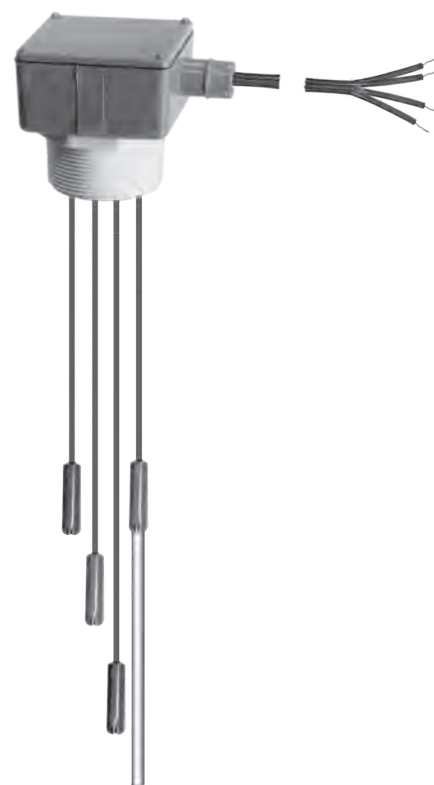
Adjustable electrode probe system (stilling chamber removed)
