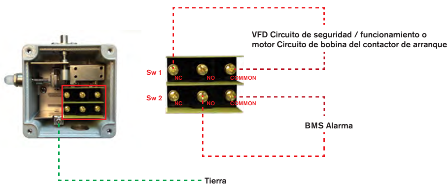
Typical output contact wiring
