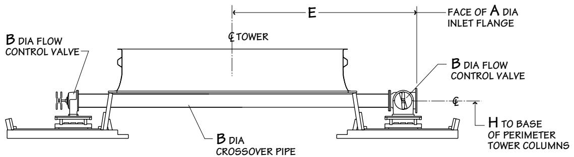
SECTION-DISTRIBUTION SYSTEM
