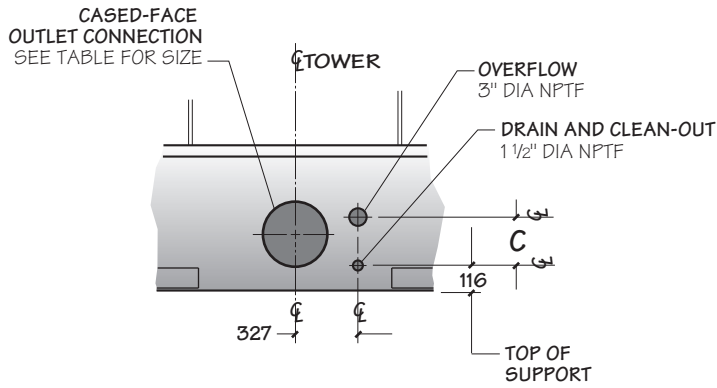
DRAIN AND OVERFLOW CONNECTION OPTION
