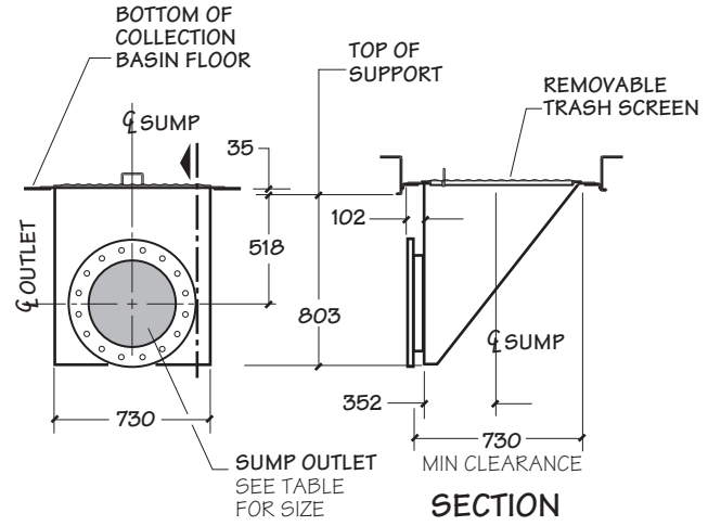
DEPRESSED SIDE-OUTLET FLANGED SUMP CONNECTION 16" AND 18" DIAMETER
